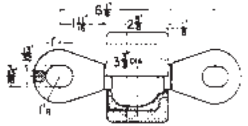
Strain Type 61348
