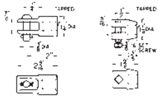
90809 — 1/2" Pin Type 63446 — 5/8" Pin Type
