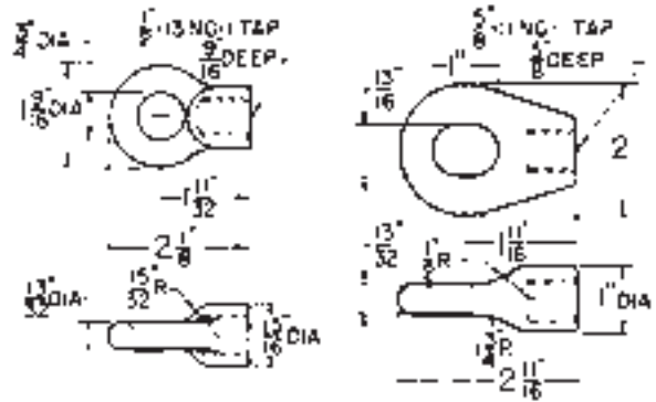
Strain Eyes
