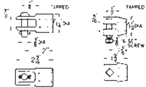
90811 — 1/2" Bolt Type 98312 — 5/8" Bolt Type
