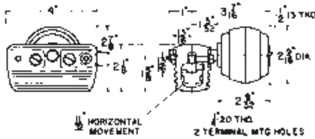
Single XVI with Insulator Mounting
