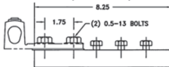
CATALOG NUMBER 106170 (1-LUG PROVISION)
