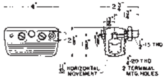
Collector Unit only with Threaded Stud
