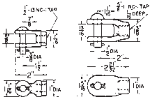
Strain Clevises
