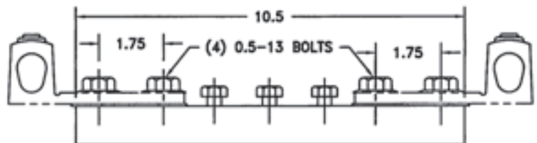
CATALOG NUMBER 106171 (2-LUG PROVISION)
